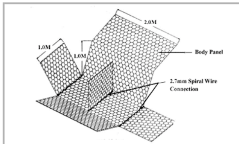
Construction Drawing of Camel Brand Standard 2x1x1m Gabion
